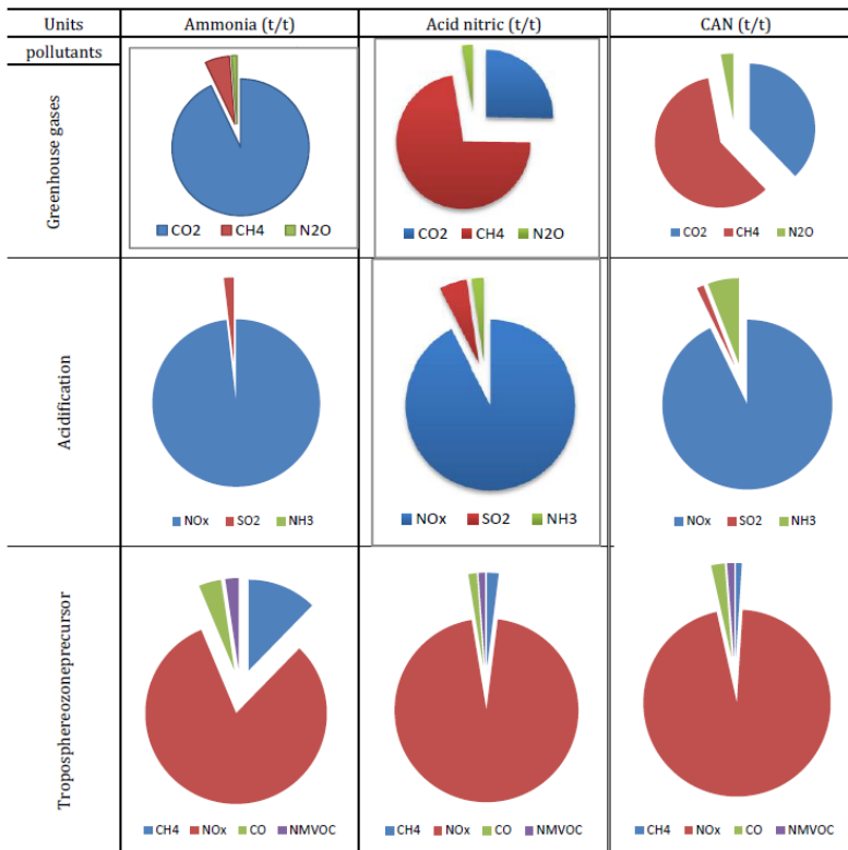
Figure.1. Emission factors in the impact categories in the process of each unit
