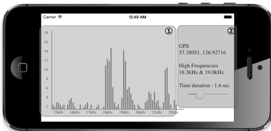
Fig. 3. Screen composition of the proposed application for assigning sequence numbers to customers
