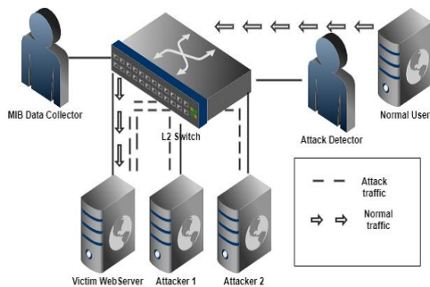
Fig 3: LDoS Testbed
