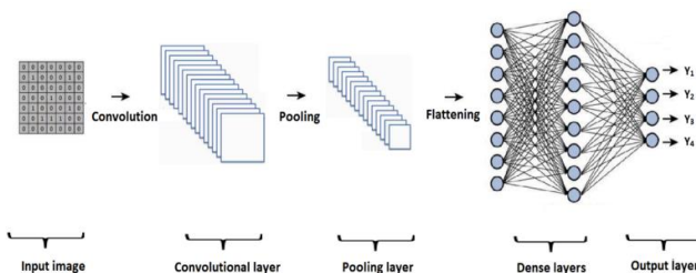
Fig. 2. CNN Architecture
